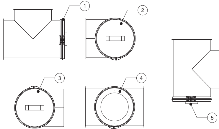
Figure 14 - Tee Position
