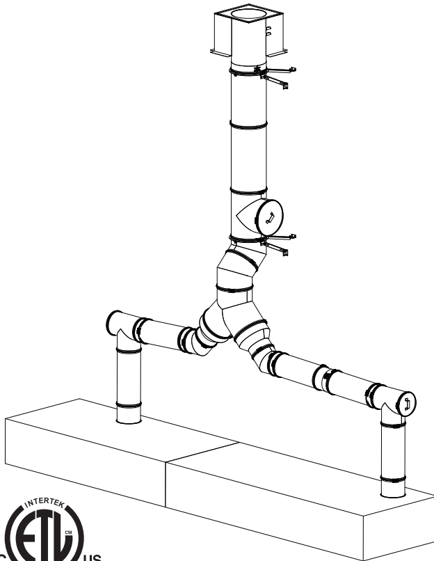
Grease Duct
