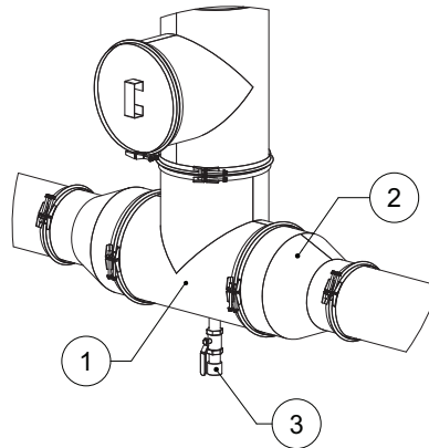
Figure 12 - Drain
