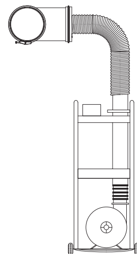
Figure 32 - Leakage Test
